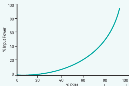
PUMP MOTOR SPEED VS. POWER CONSUMPTION
