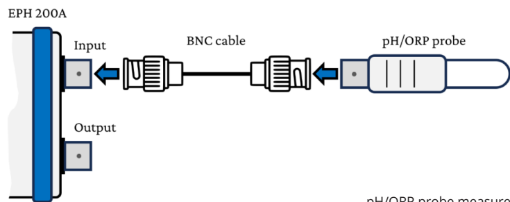
pH/ORP probe measurement
